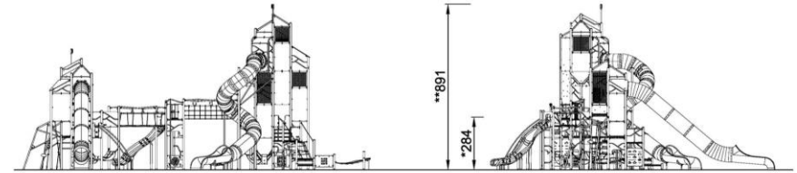
PCT310101 1:300
